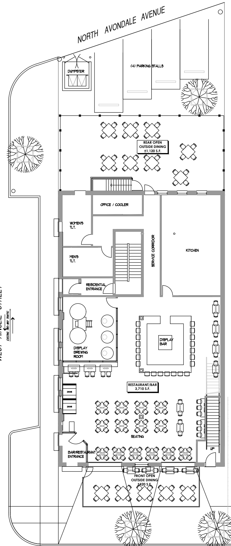
PROPOSED DD1.1 FIRST FLOOR PLAN
