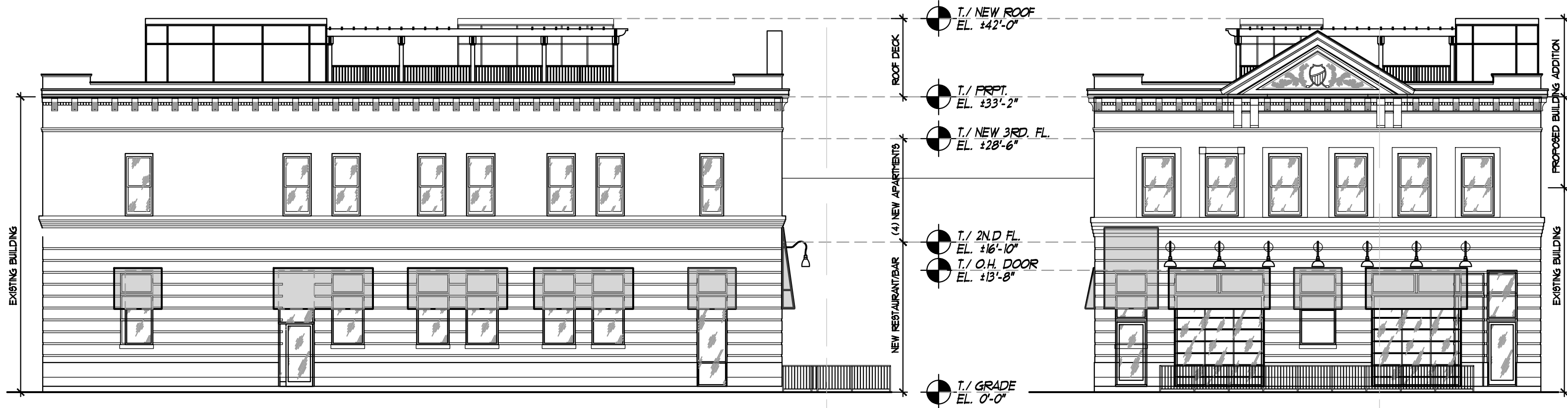
PROPOSED DD1.1 NORTH BUILDING ELEVATION
